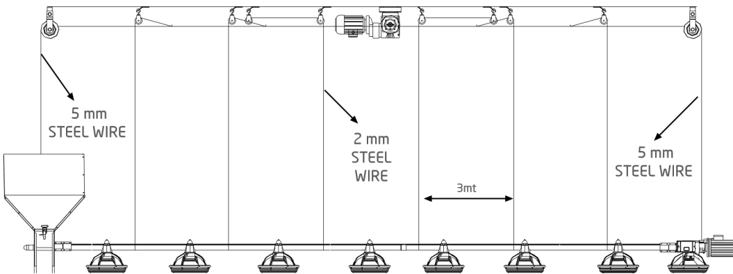
Motored Winch
